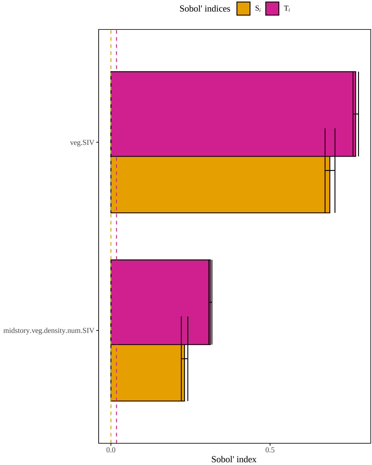
Figure 5. Results of a sensitivity analysis for the cactuswren model based on a geometric mean structure. Dashed lines represent baseline numerical approximation error for S_i and T_i ( i.e. , dummy variables).
